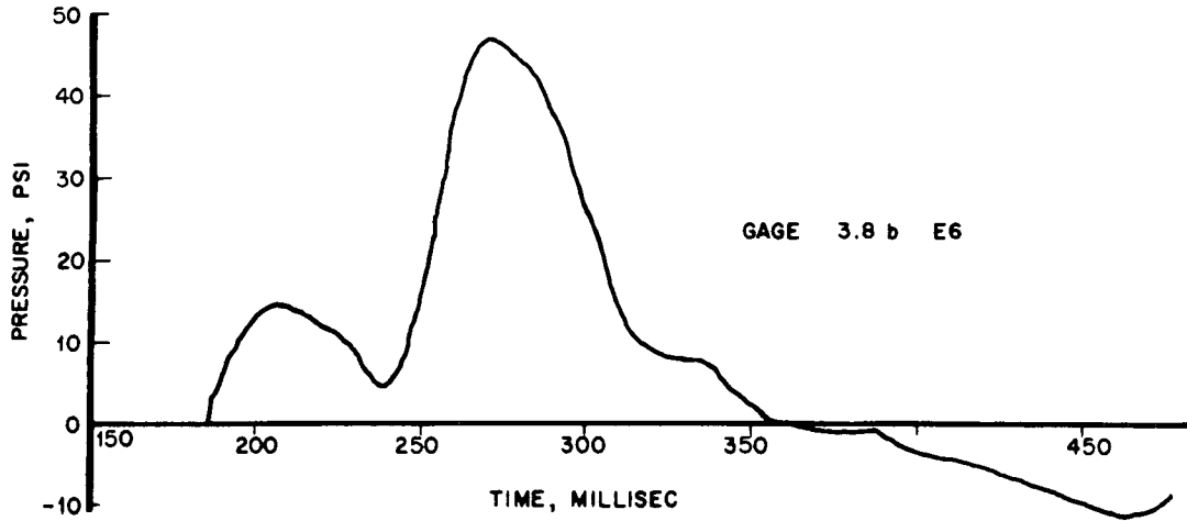
Fig. 12—Base pressure on structure 3.8b.
